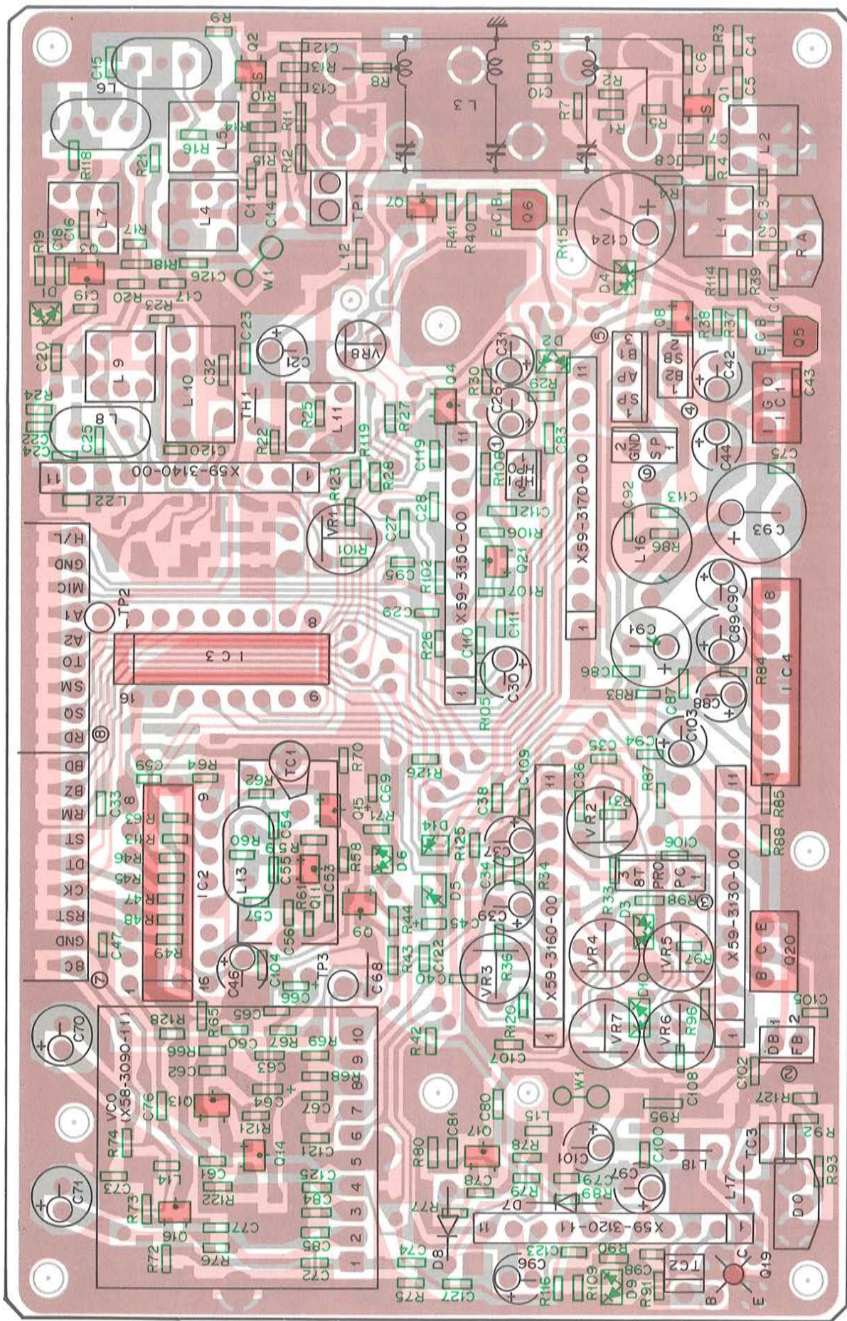
TX-RX UNIT (X57-3170-10) Foil side view
