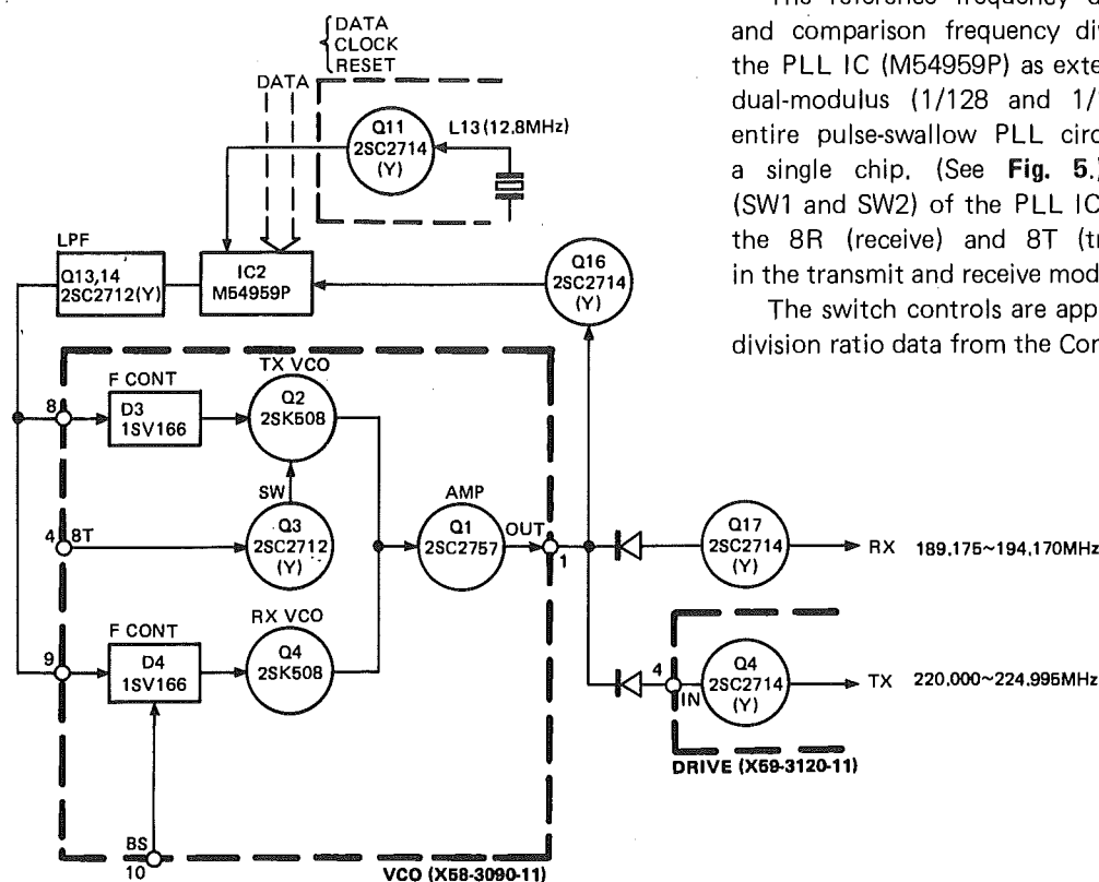
Fig. 4 PLL system block diagram
