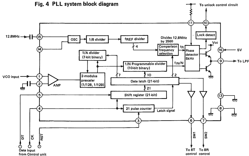
Fig. 5 PLL IC ; M54959P block diagram
