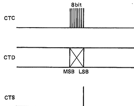
Fig. 16 CTCSS data transfer format
