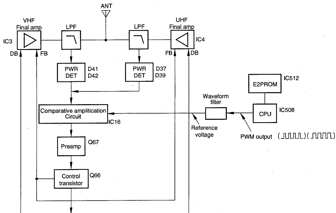
Fig.2 APC circuit
