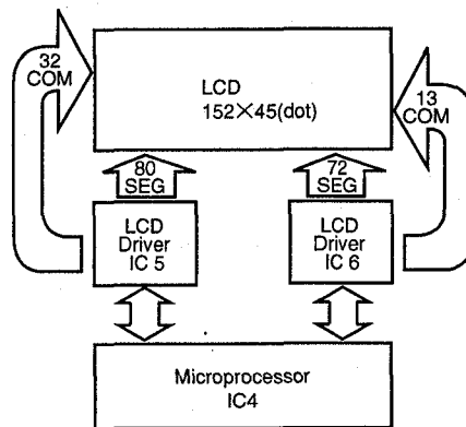
Fig.16 Display circuit
