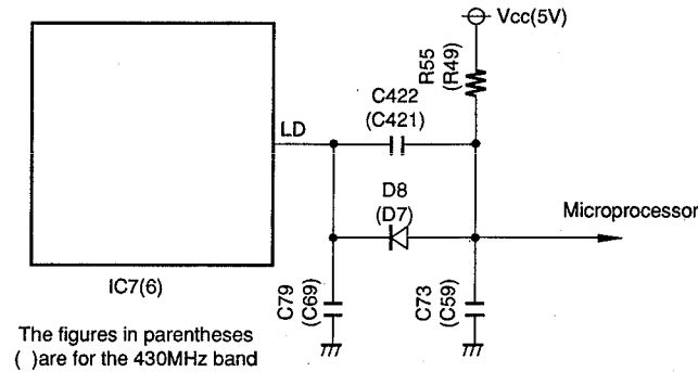
Fig.5 Unlock circuit
