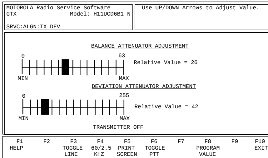
Figure 3-4. Transmitter Deviation Adjustment
