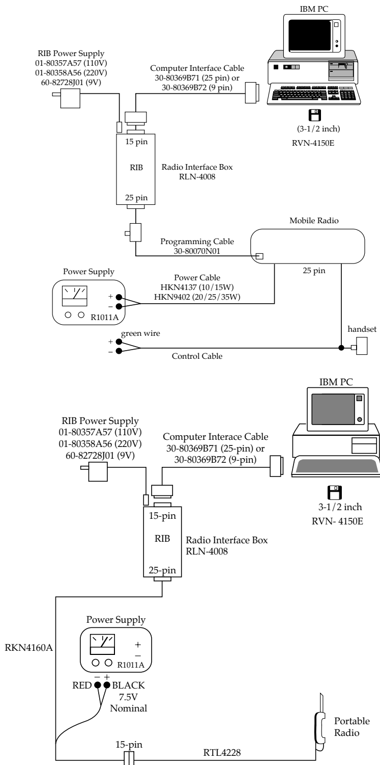
Figure 2-1. Radio-RIB-Computer Configuration
