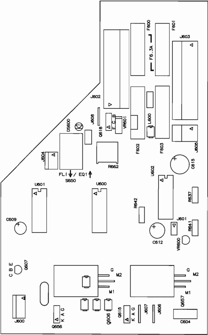
COMPONENT SIDE
