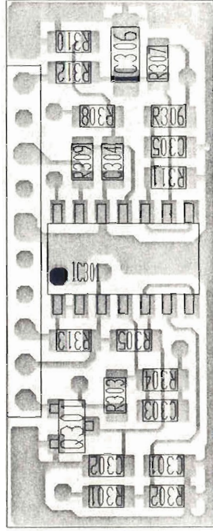
(Top View)
