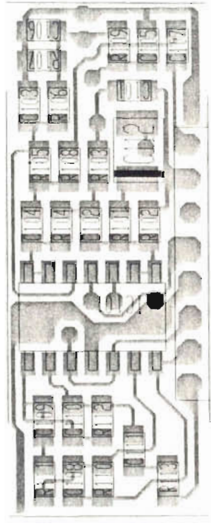
(Top View)
