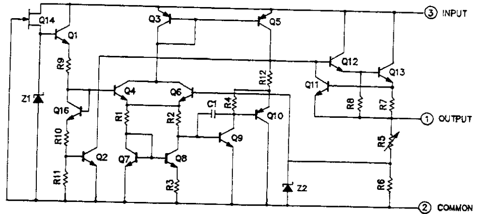
Equivalent Circuit
