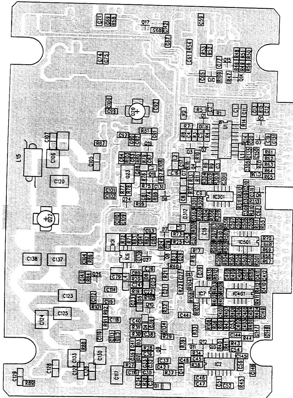
Bottom View
