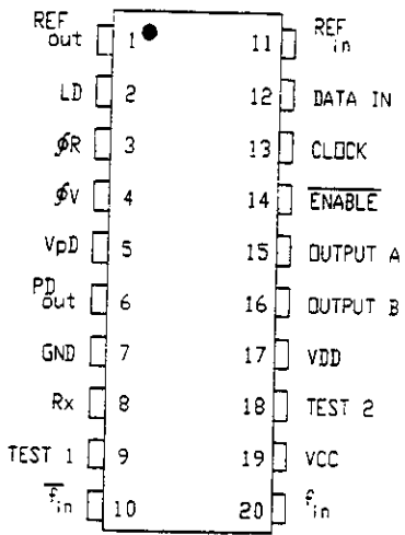
Pin Connection
