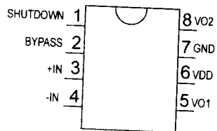
LM4864MM
