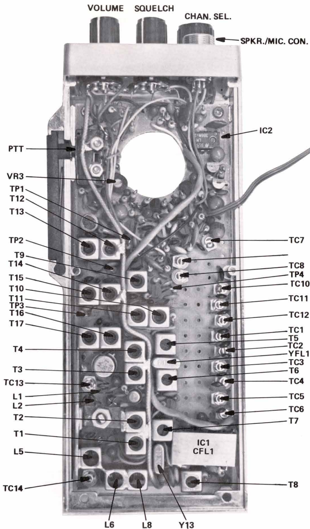
FIGURE 5-4 PARTS PLACEMENT
