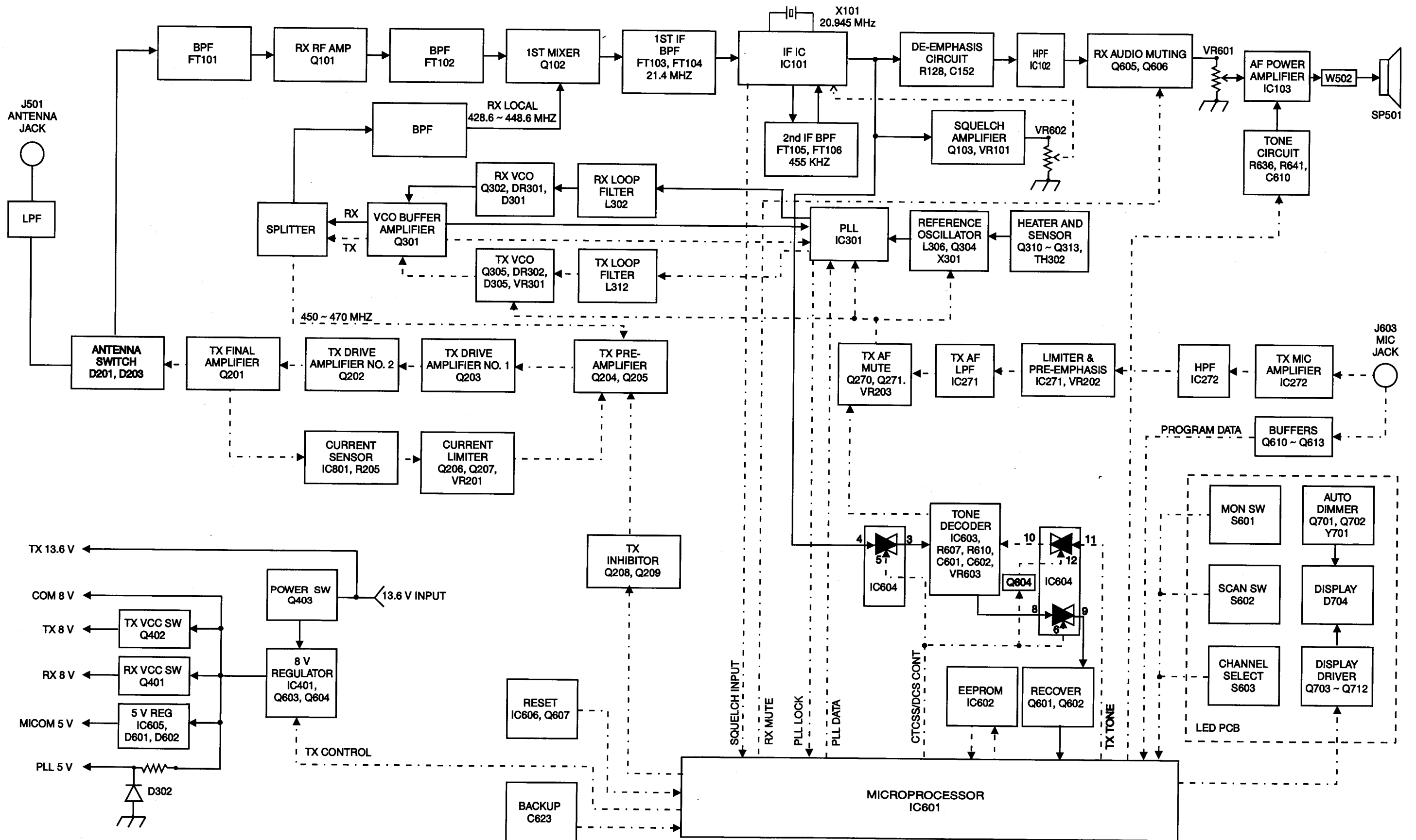
Block Diagram
