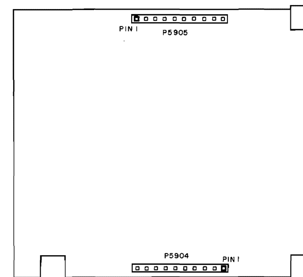
GP1B ANALYZER DIGITIZER PC BOARD
