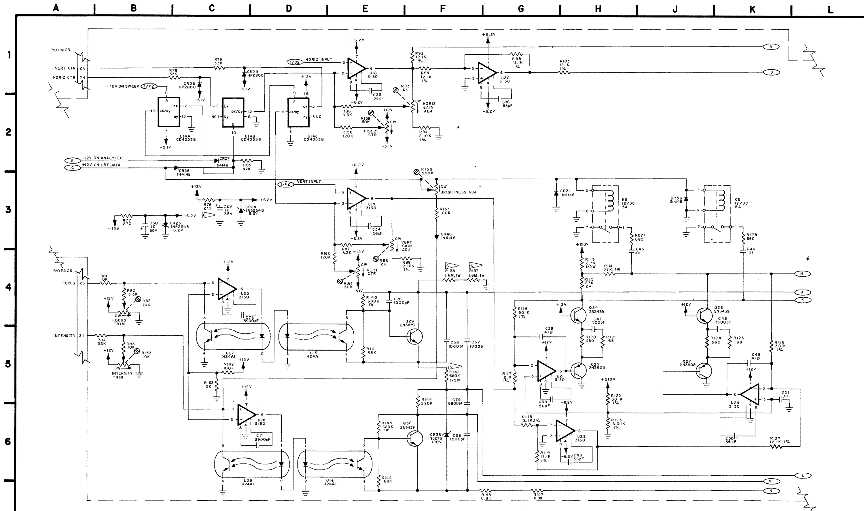
Figure 7-25 Oscilloscope Control and Deflection PC Board Schematic (Sheet 3 of 4) 0000-5015-100-G1
