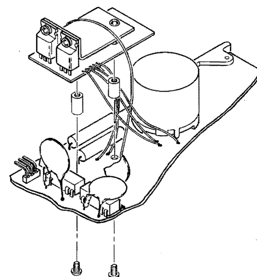
OSCILLOSCOPE CONTROL AND DEFLECTION PC BD WITH INVERTER ASSY
