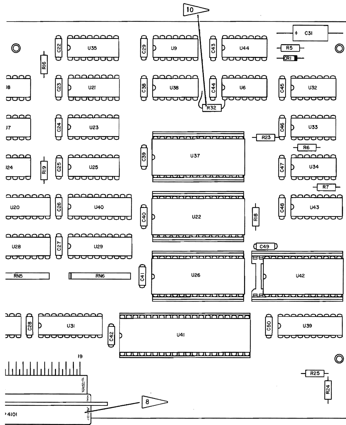
(THRU SER. NO. 2060) (7010-5034-100-C3) TOP VIEW
