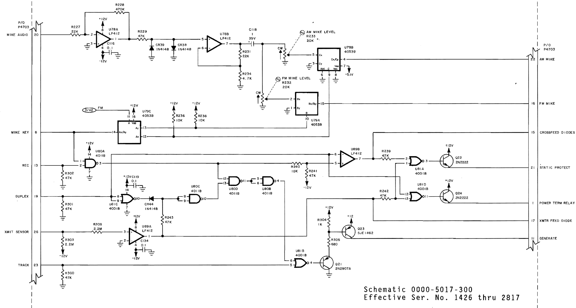
Figure 7-24a Demond Audio PC Board Schematic (Sheet 7 of 12) 0000-5017-300-D1 0000-5018-900-A
