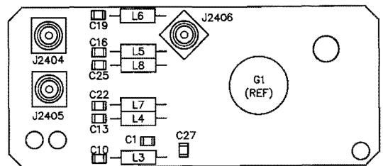
1300-2300 MHz VCO PC BD
