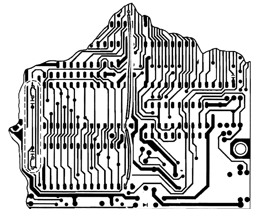
TOP VIEW GPIB - CELLULAR OPTION (7010-5034-102) THRU SER. NO. 2060
