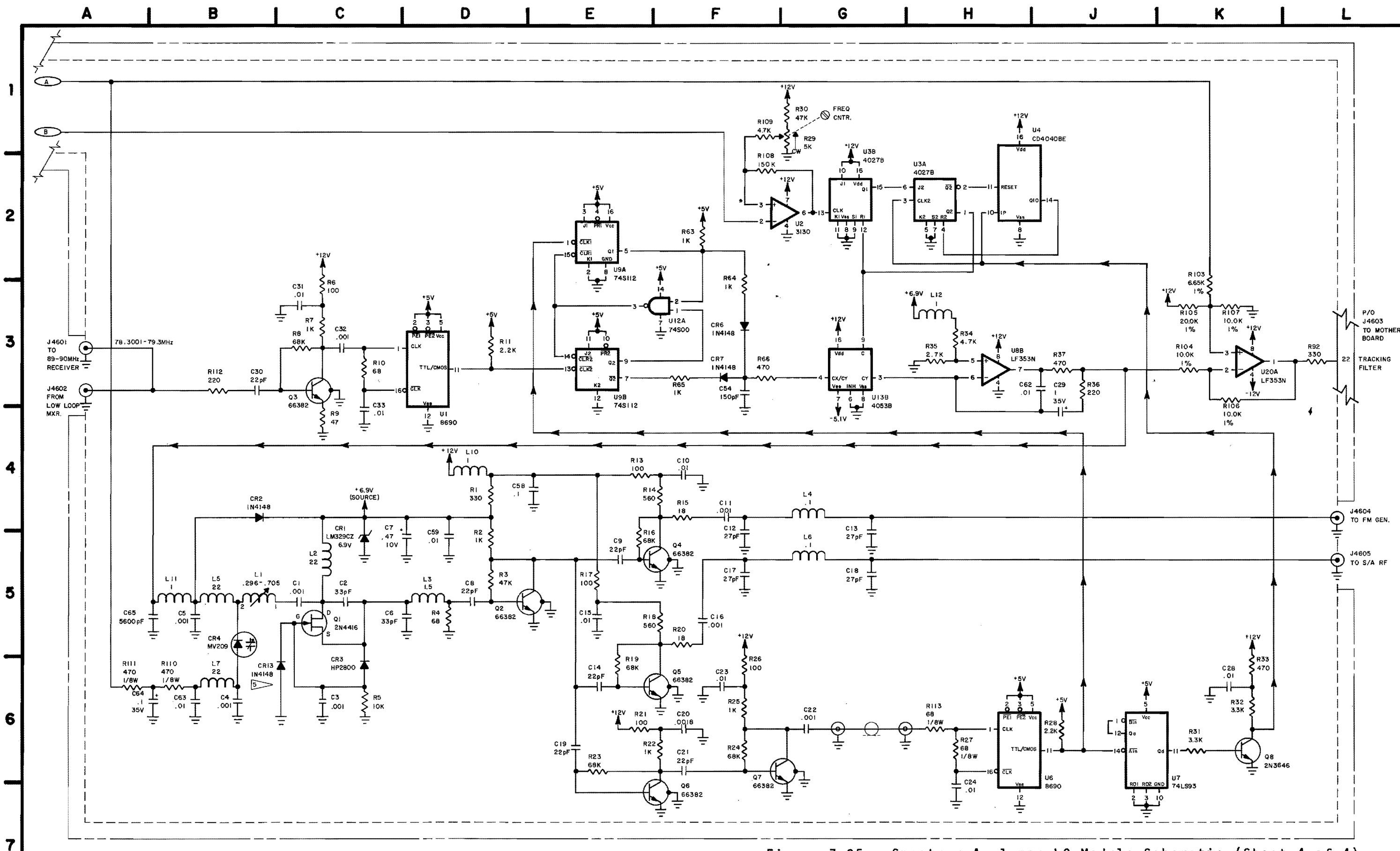
Figure 7-35 Spectrum Analyzer LO Module Schematic (Sheet 4 of 4) 0000-5013-500-F5
