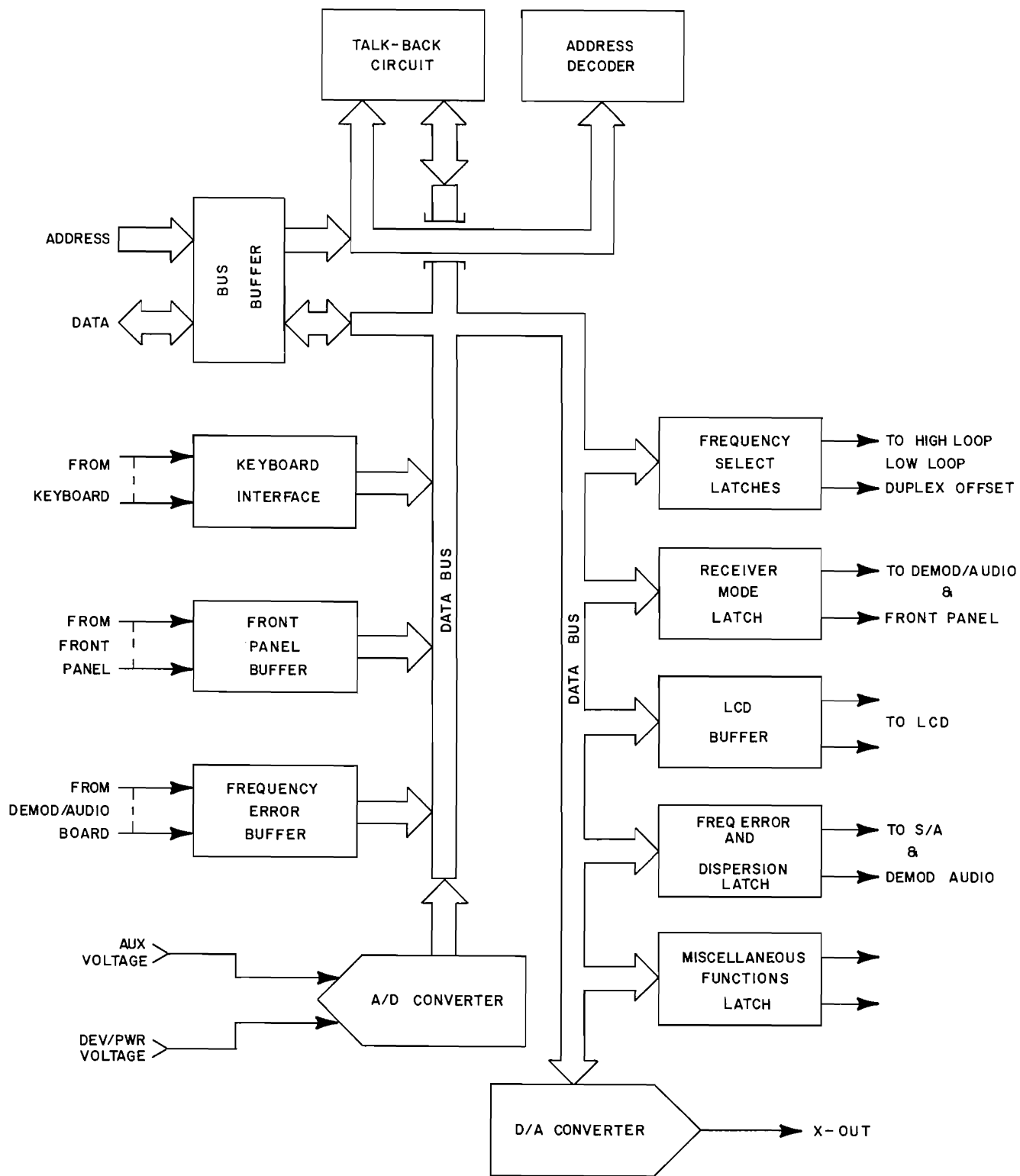
Figure 2-31 I/O Interface PC Board Detailed Block Diagram
