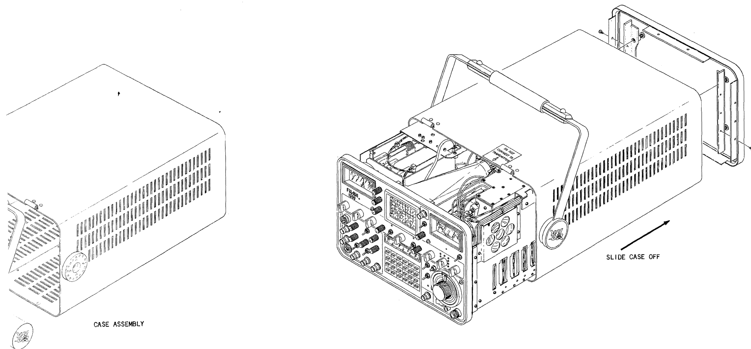
Figure 6-1 Composite Assembly (Sheet 1 of 2)
