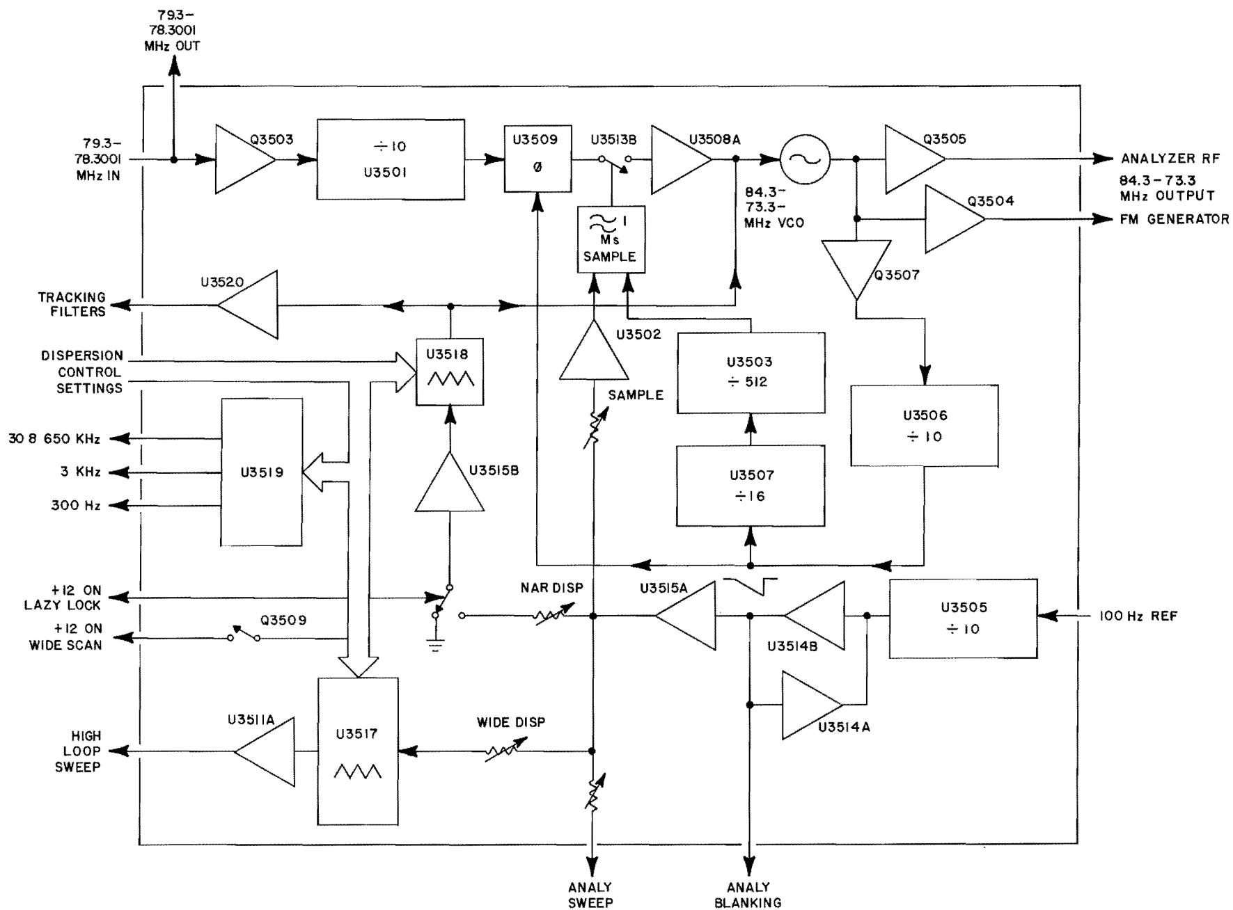
Figure 2-27 Spectrum Analyzer LO Detailed Block Diagram
