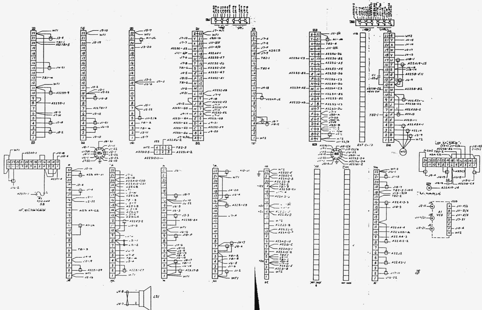
Figure 6-23. Interconnection Diagram, Main Chassis. A24 6-107/6-108
