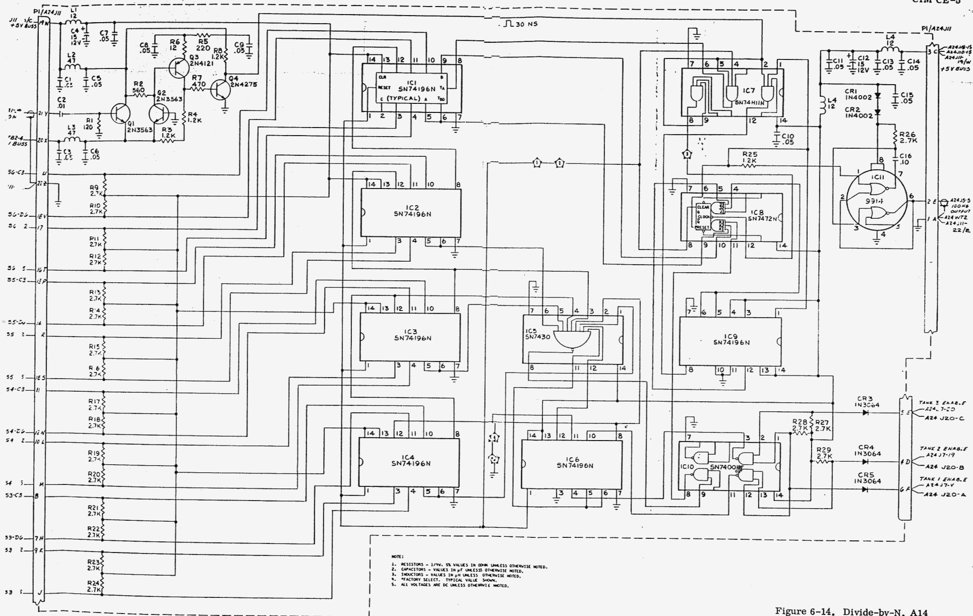
Figure 6-14. Divide-by-N, A14
