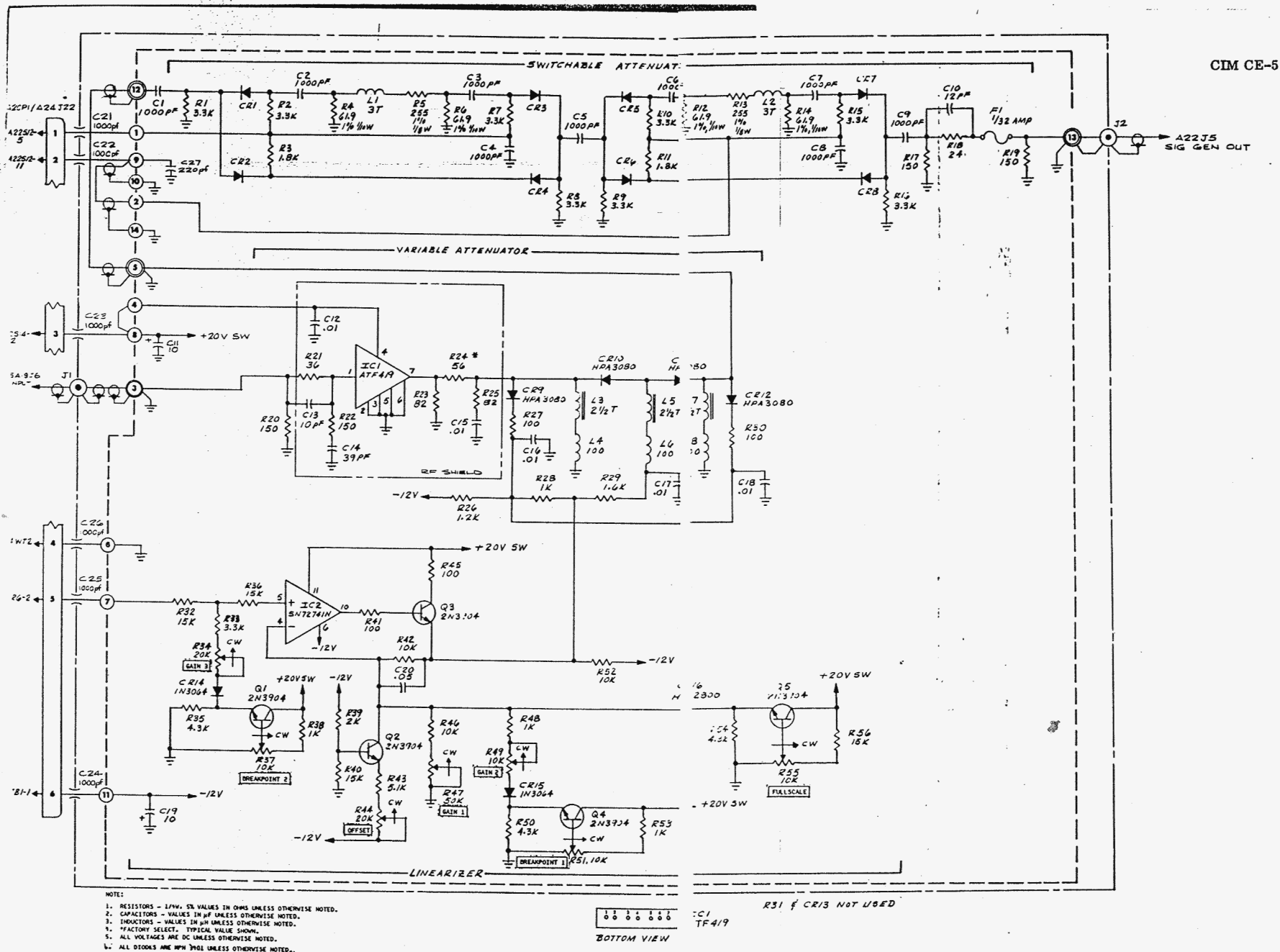
Figure 6-26. Output Attenuator. A20
