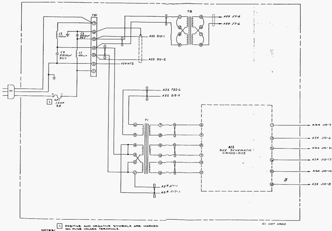
Figure 6-22, Wiring Diagram, Rear Panel. A23
