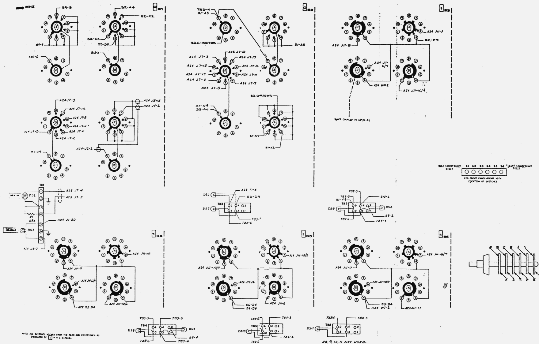
Figure 6-20. Interconnection Diagram, Front Panel, Sheet 1. A22 6-97/6-98
