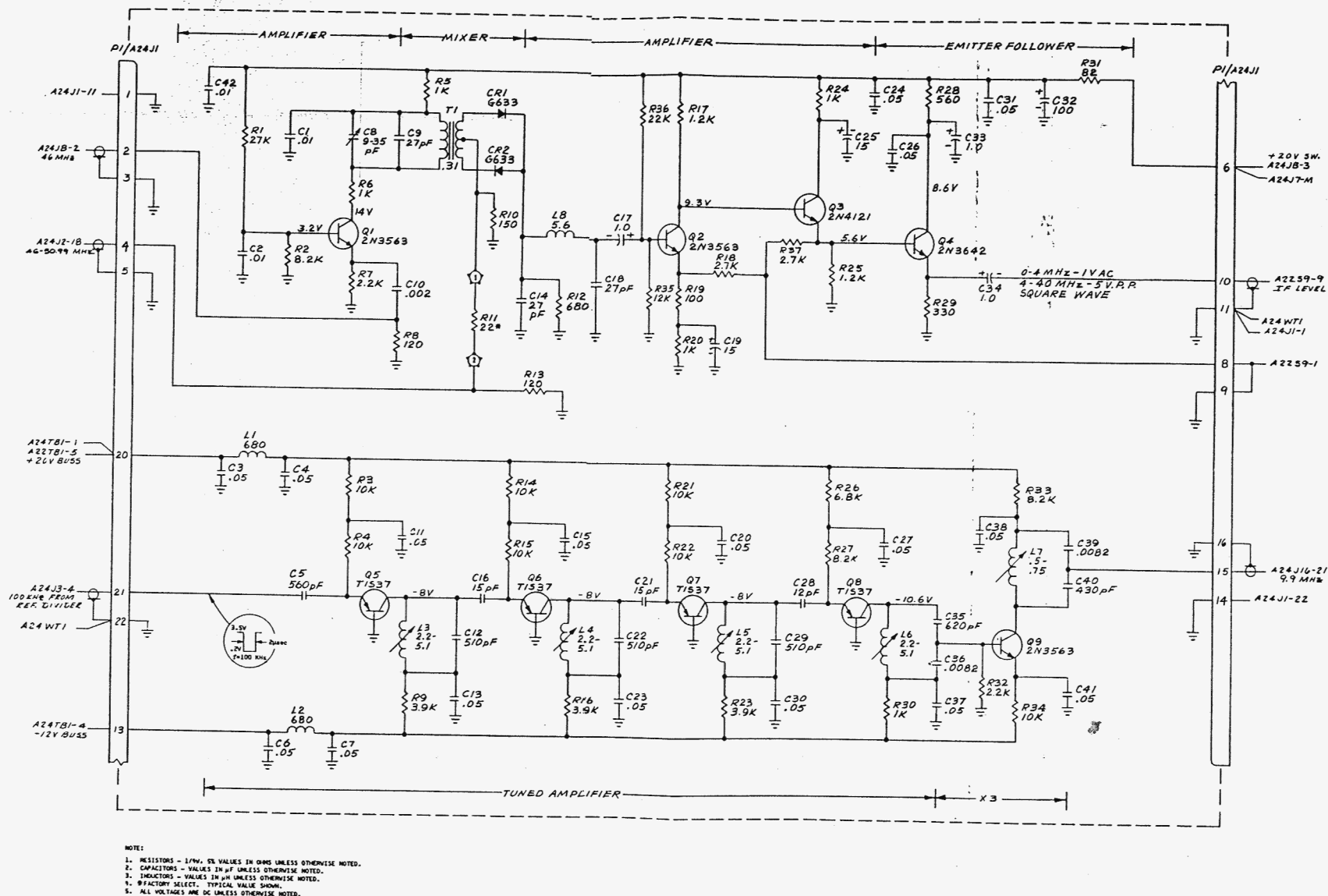
Figure 6-7. 1 kHz-4 kHz Mixer/9.9 MHz Filter, A7
