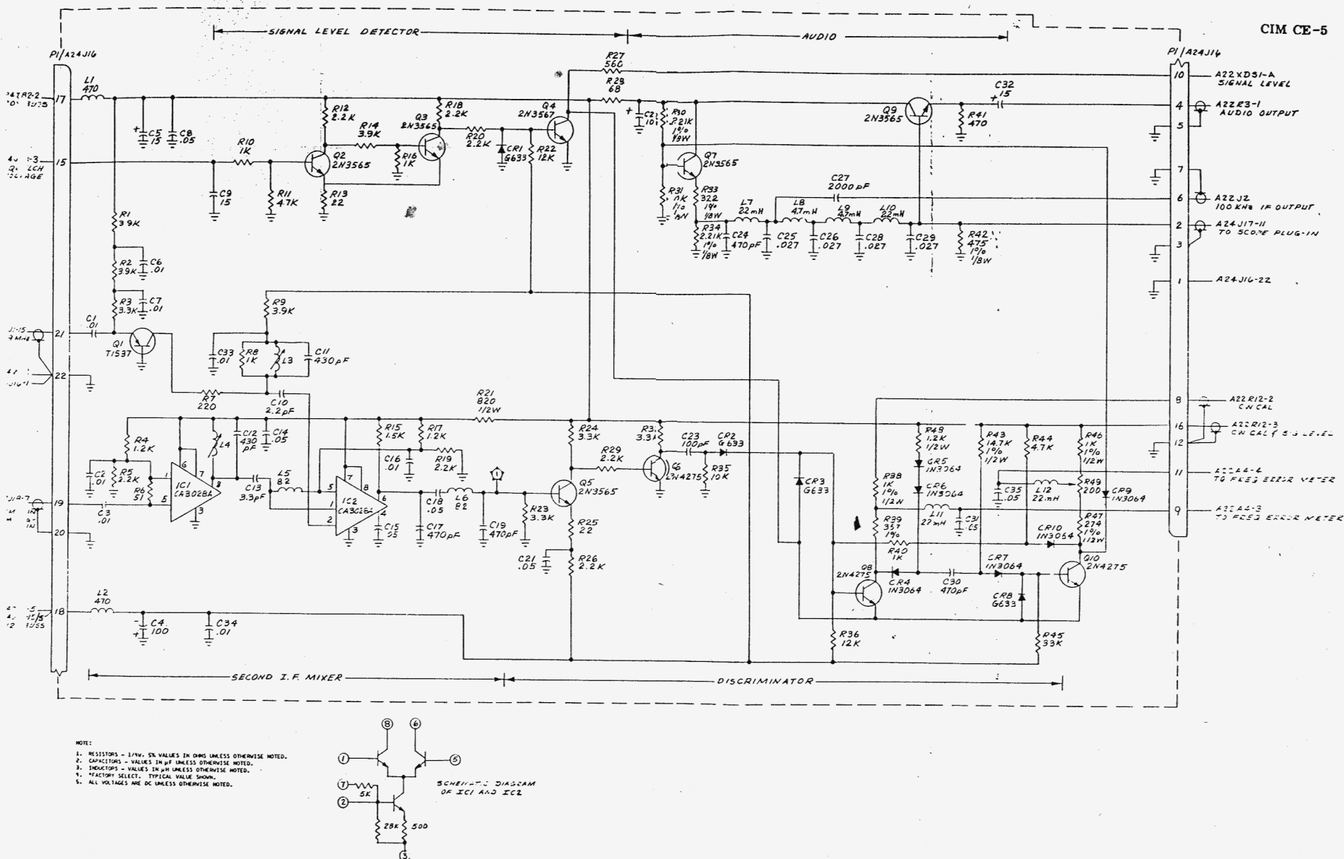
Figure 6-5. Second IF/Discriminator, A5
