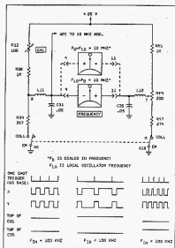
Figure 4-5. Frequency Meter Bridge Circuit
