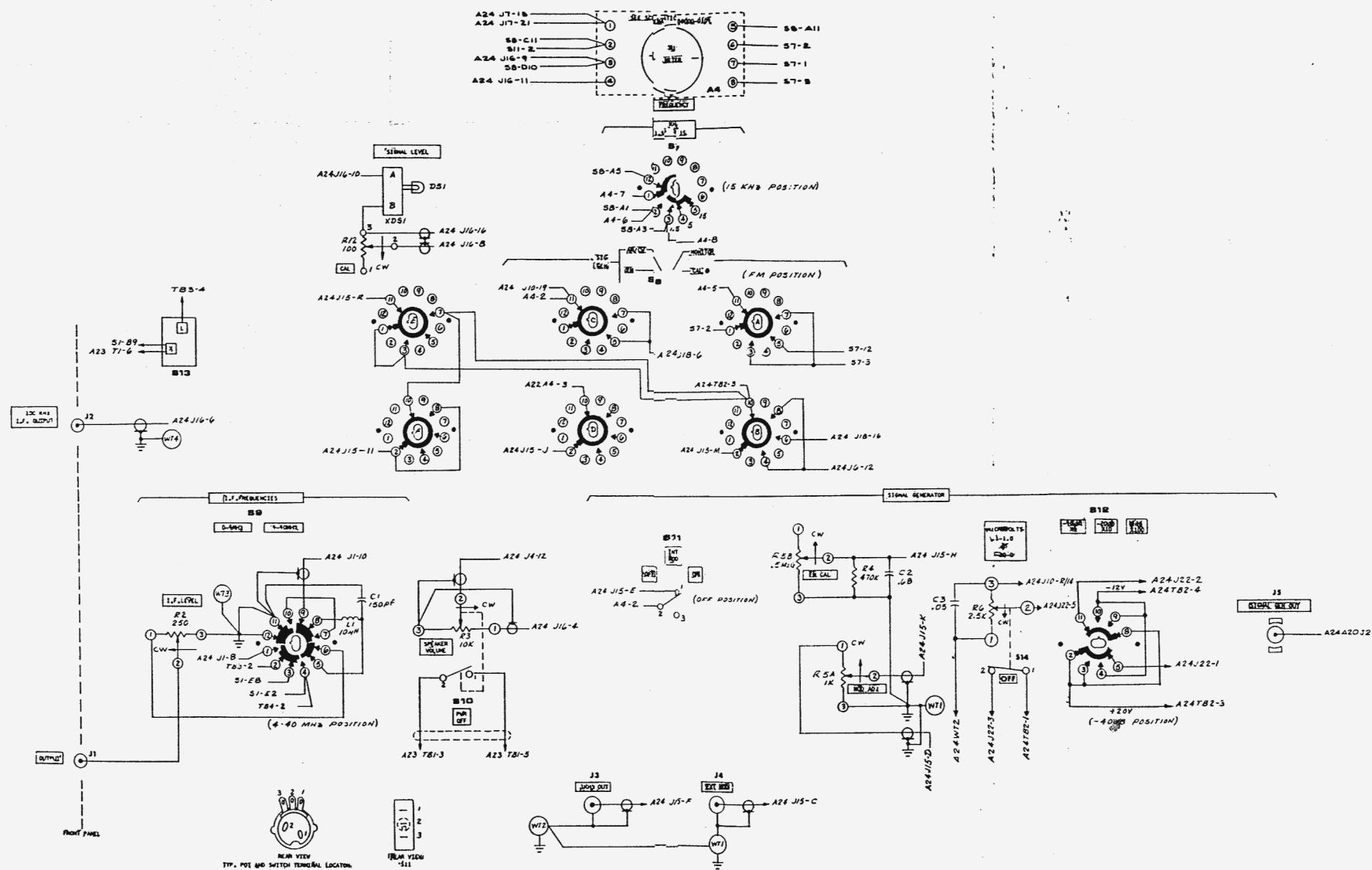
Figure 6-21. Interconnection Diagram, Front Panel, Sheet 2. A22 6-99/6-100
