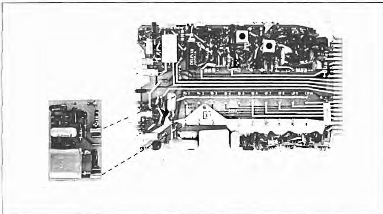
Figure 3-1. Installation-Removal, IF-Oscillator Boards
