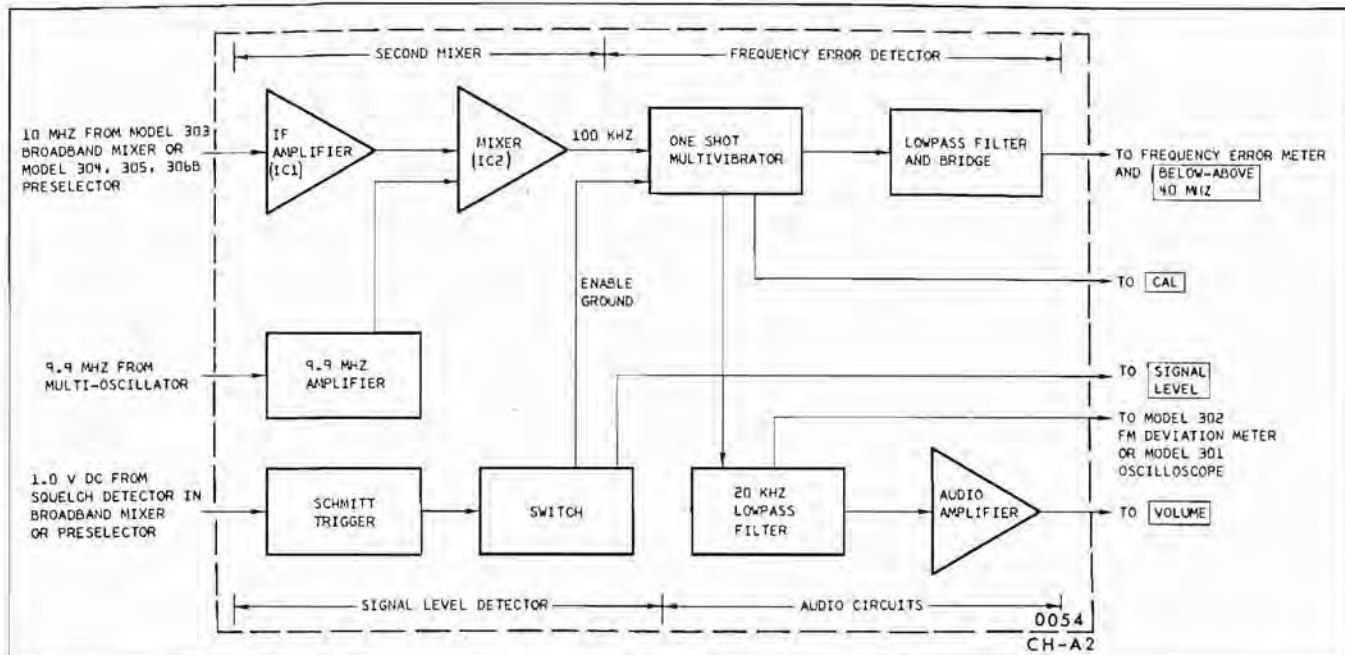
Figure 4-2. Second IF and Discriminator Board, Block Diagram
