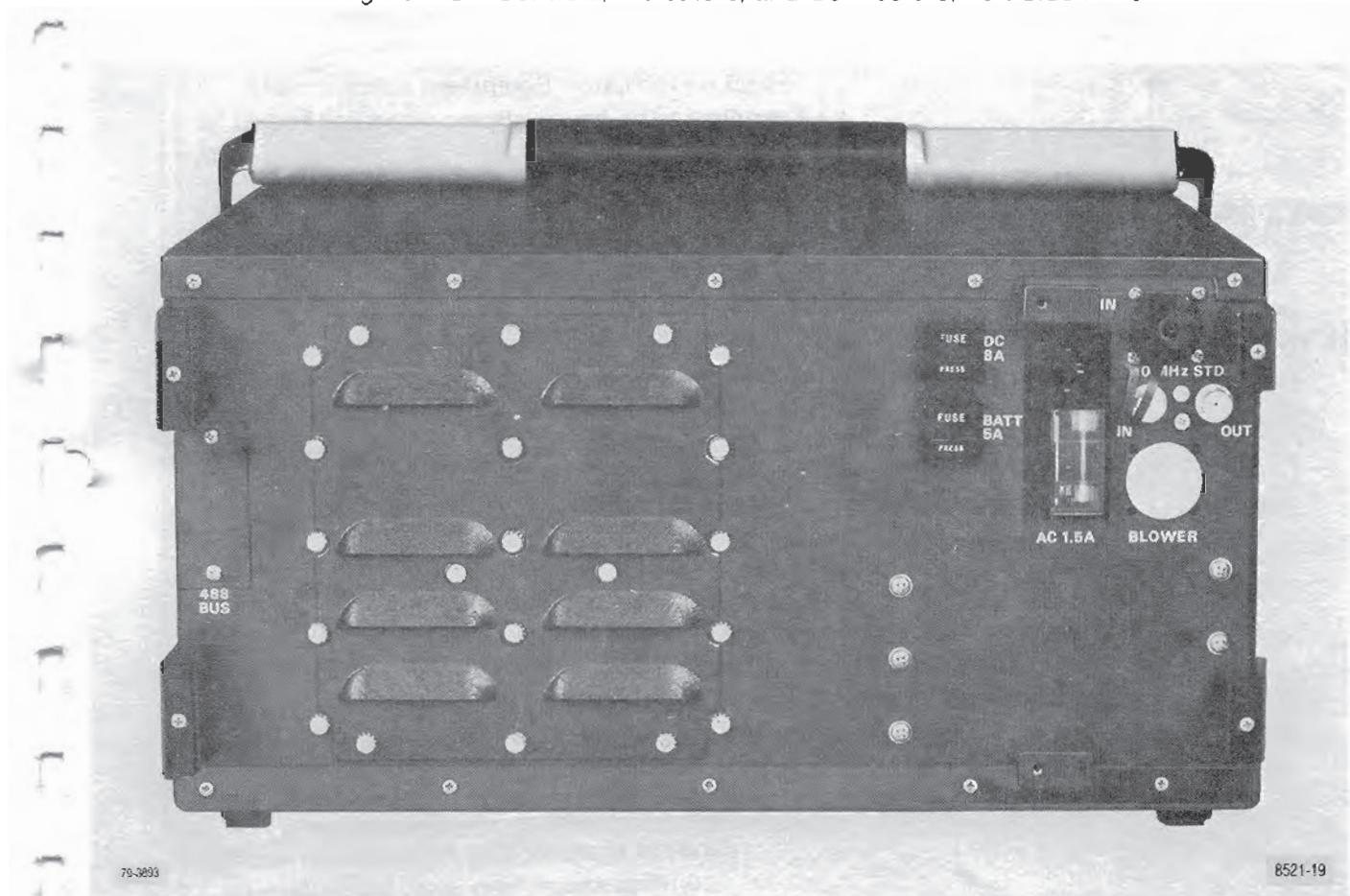
Figure 4-3. Controls, Indicators, and Connectors, Rear Panel
