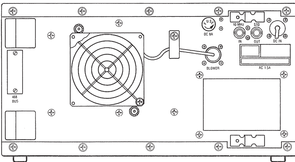
Figure 4-3. Controls, Indicators, and Connectors, Rear Panel
