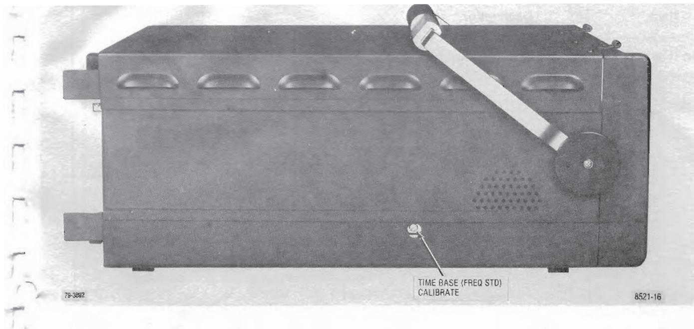
Figure 4-2. Controls, Indicators, and Connectors, Left Side Panel
