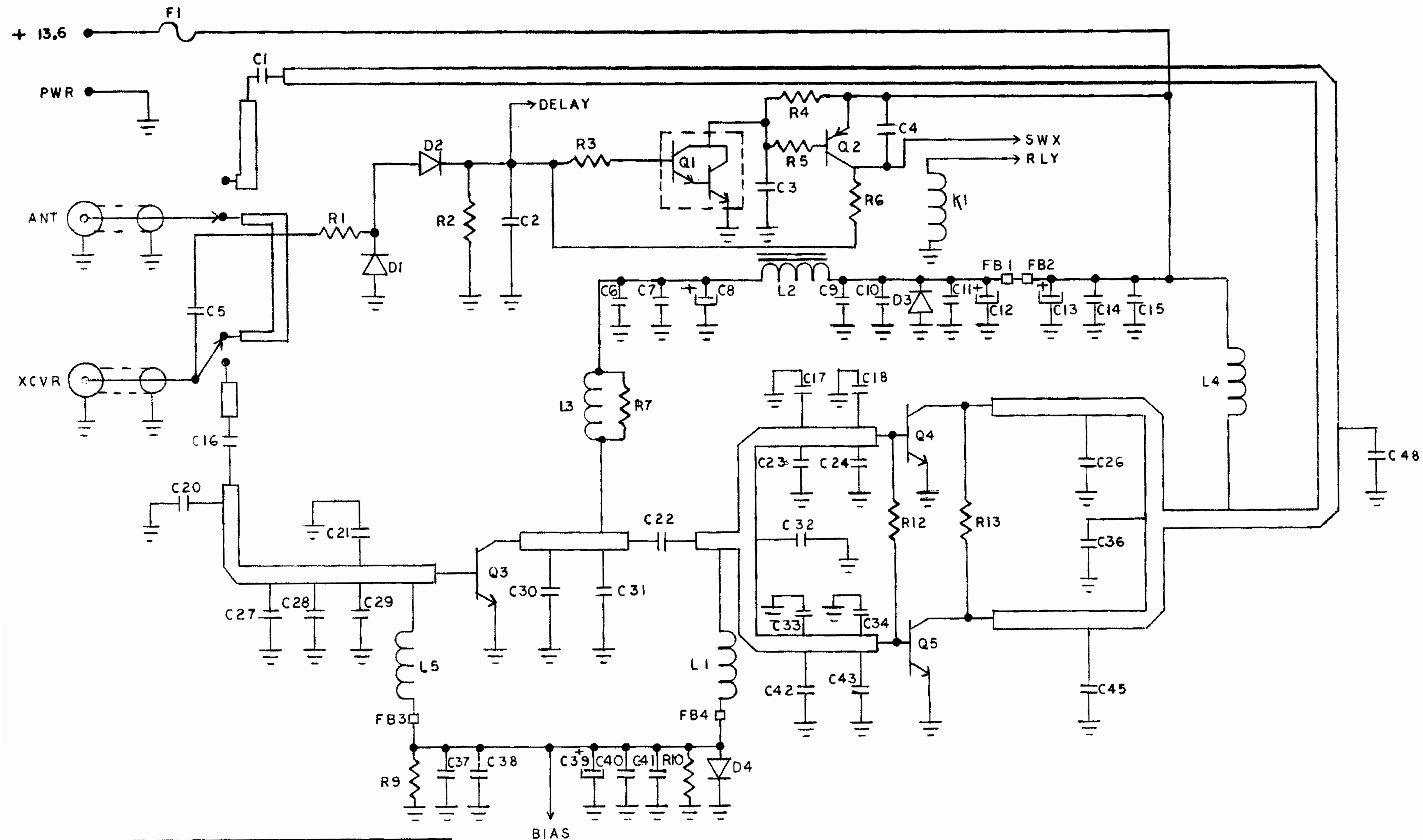
BLC 10/150 BLC 30/150 SCHEMATIC DIAGRAM
