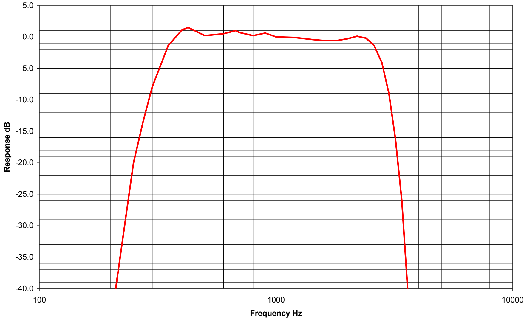
Filter Response
