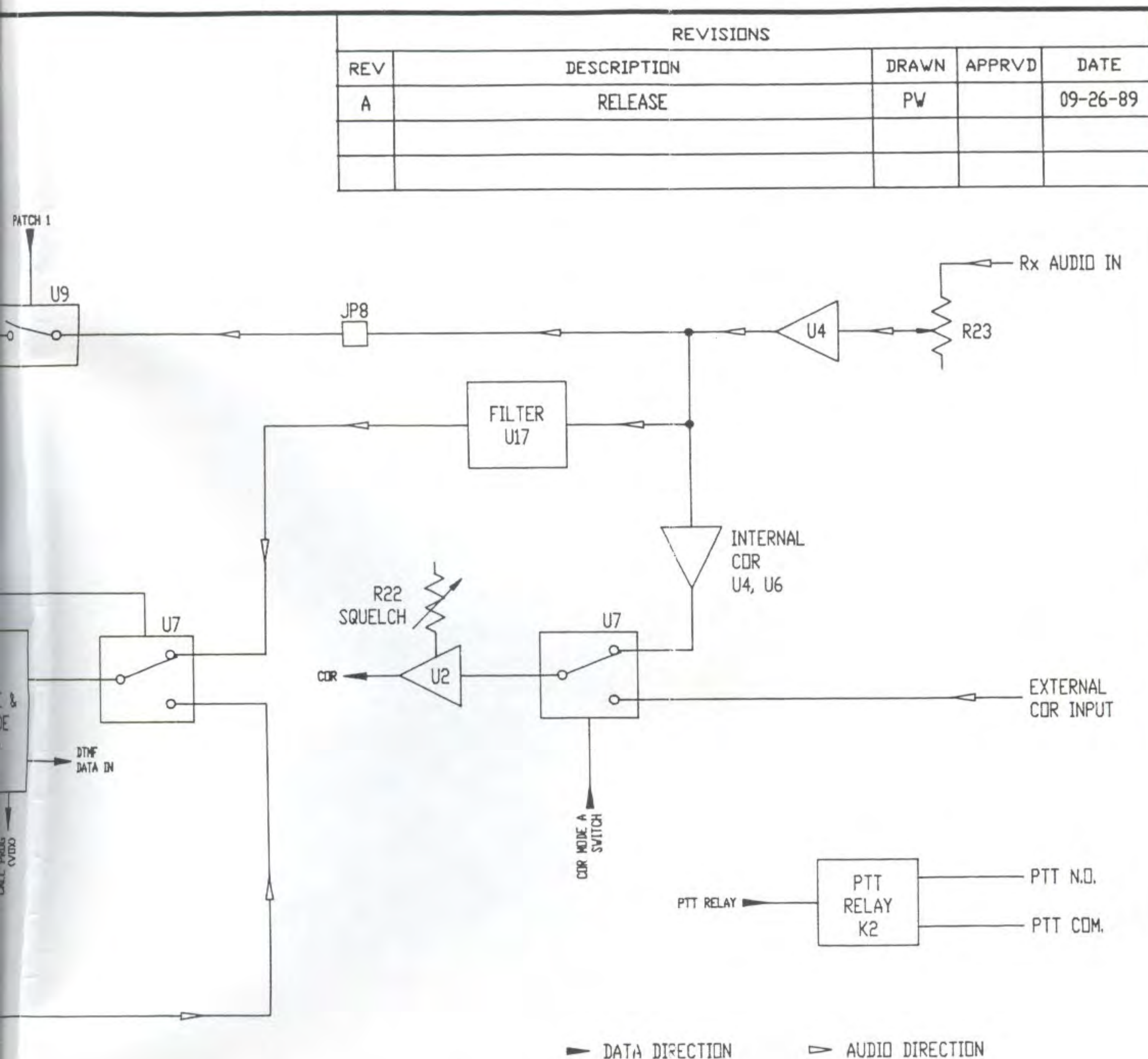
MODEL 35A BLOCK DIAGRAM (006-0054A)
